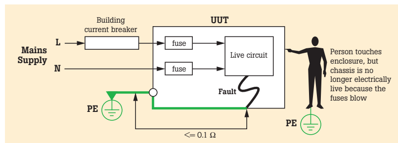
Figure 7. Appliance current fault protection.
