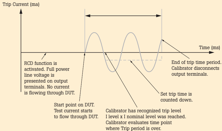
Figure 12. Timing of the RCD calibrator, which acts as a highly accurate, variable RCD.
