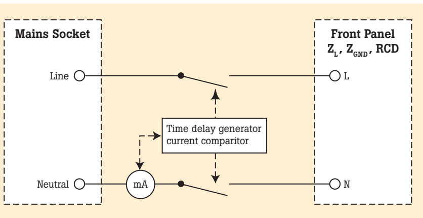
Figure 11. The block diagram of the RCD function in the calibrator. [5]
