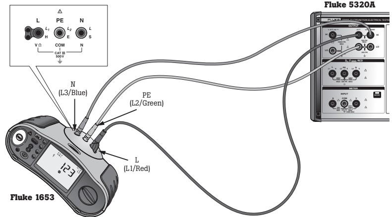
Figure 6. Testing a three-pole earth resistance tester with the calibrator [5].
