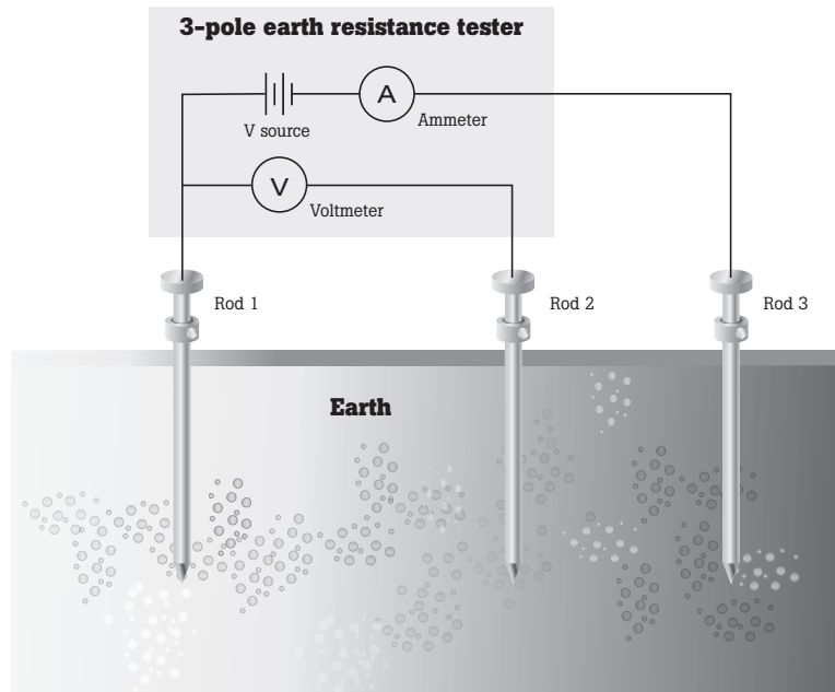
Figure 4. A 3-pole tester works by providing a known current through an earth path, from Rod 3 to Rod 1. In the fall-of-potential resistance test, the resulting voltage is measured at various points of the path back to the electrode being tested.
