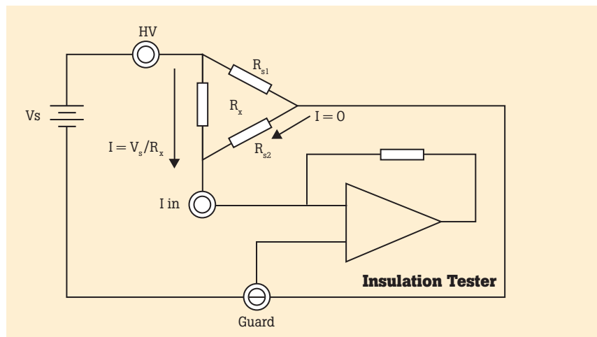
Figure 2. The guard maintains zero volts across R_{s2} , giving no current flow. All of the stimulus current flows through R_x , as desired.
