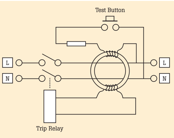
Figure 9. Block diagram of a typical RCD.
