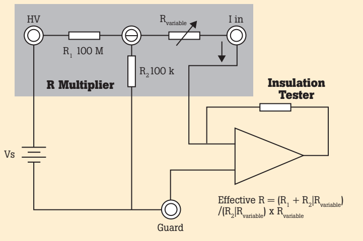
Figure 3. With Rvariable set to 100 MΩ, the effective resistance the megohmmeter reads is 1000 times higher, or 100 GΩ.
