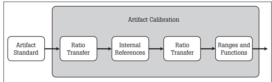
Figure 3. The traceability chain for the 5700A and 5720A
