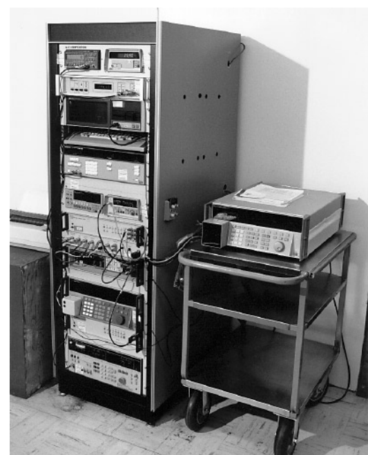
Figure 7. 5700A Automated Calibration System
